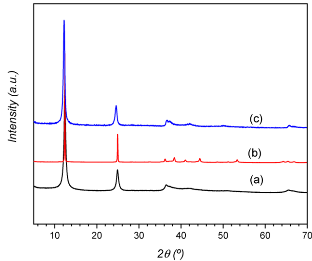
Figure 1. XRD patterns showing the (001) and (002) peaks of birnessite and their changes after interlayer cation exchange.
